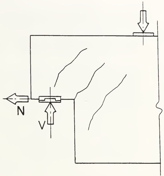
Fig. 1.5 — Typical cracking pattern of dapped-end at service load*
